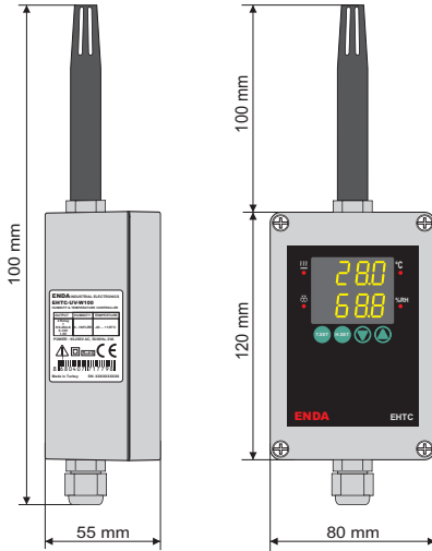
EHTC-xV-W100 WALL-MOUNTED
